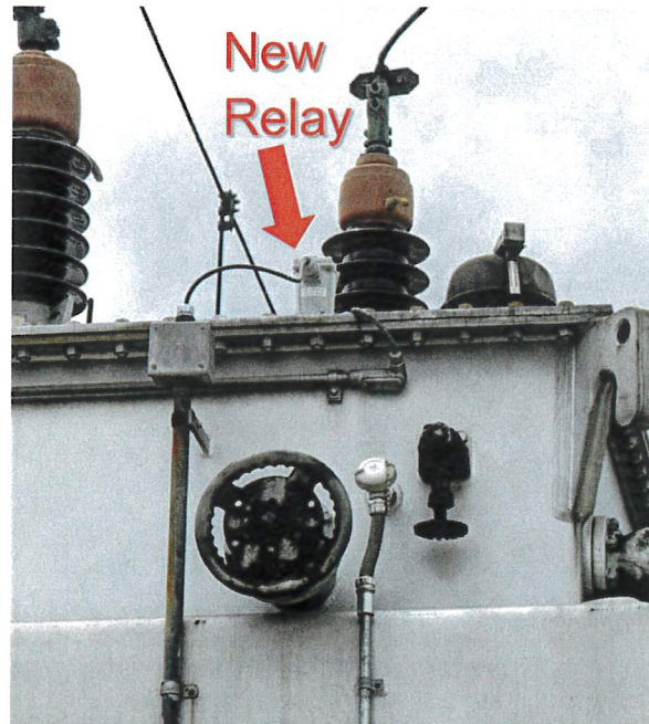
New Sudden Pressure Relays at Valley A-1
