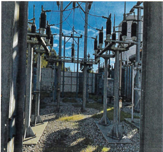
Pictures of Pacific substation prior to the demolition
