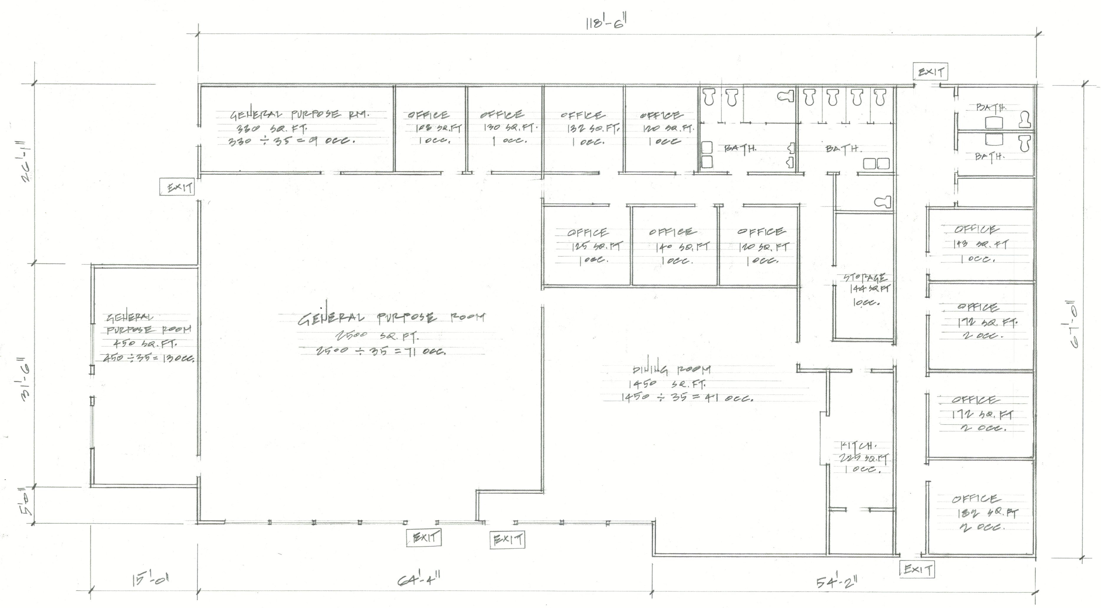
FLOOR PLAN (E)
