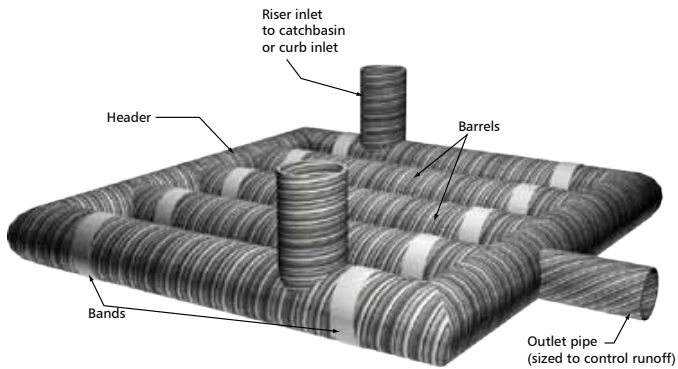
CMP detention system
