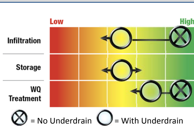
Pervious Concrete
