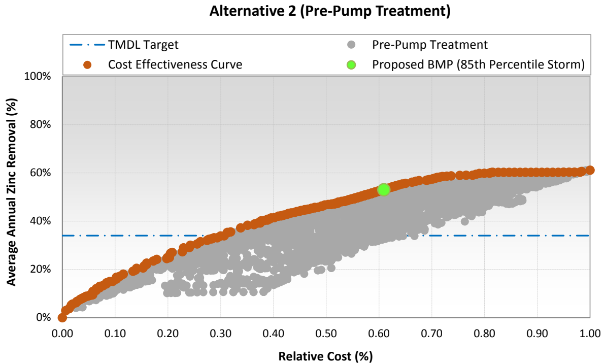
Figure 20. Relative Cost vs Average Annual Total Zinc Reduction.
