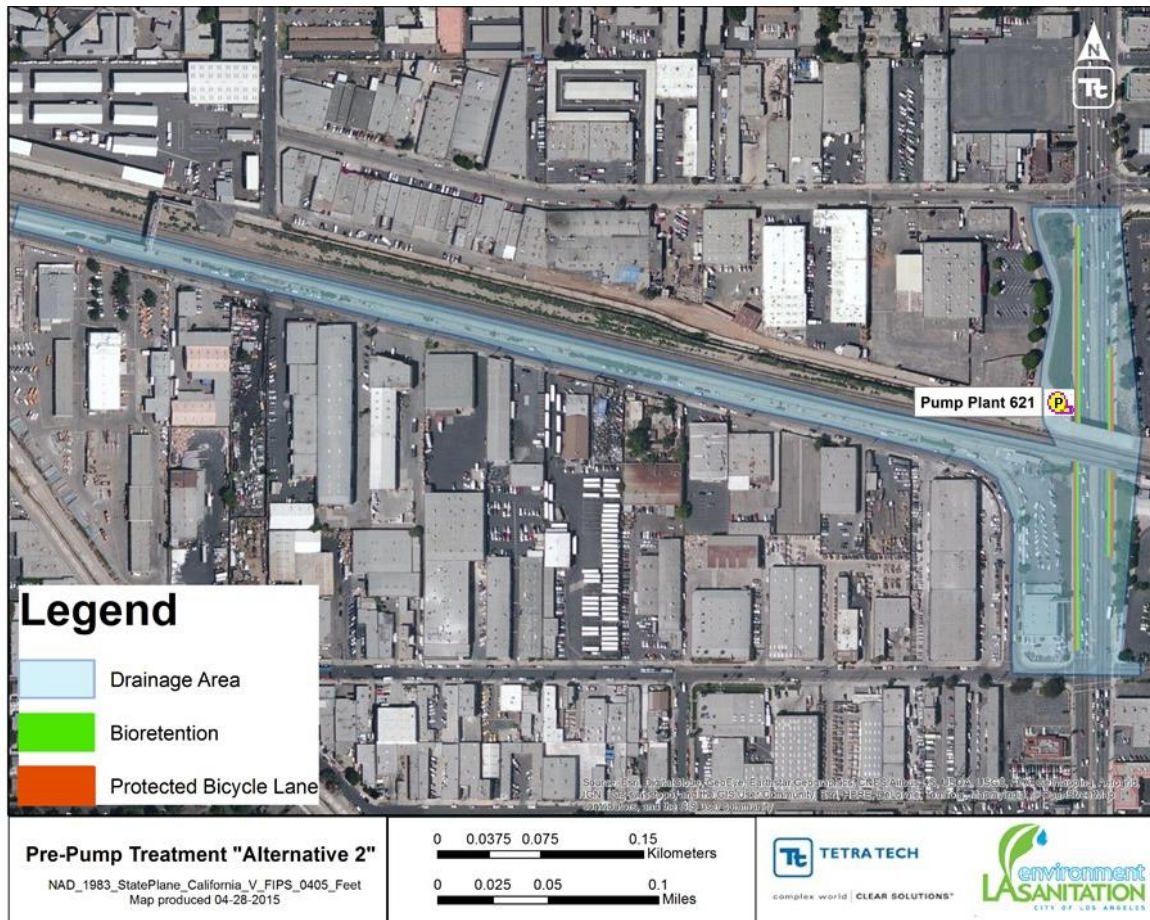
Figure 15. Alternative 2 recommended areas for BMP implementation.
