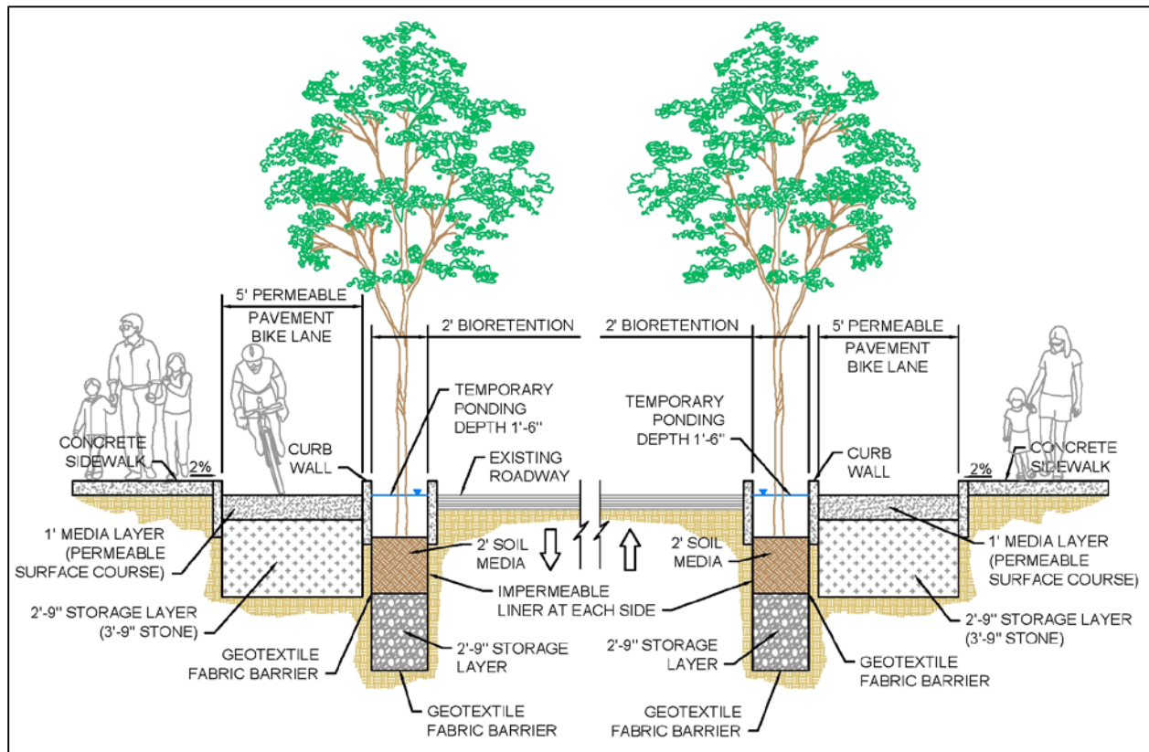
Figure 28. Expected cross section for Alternative 2.
