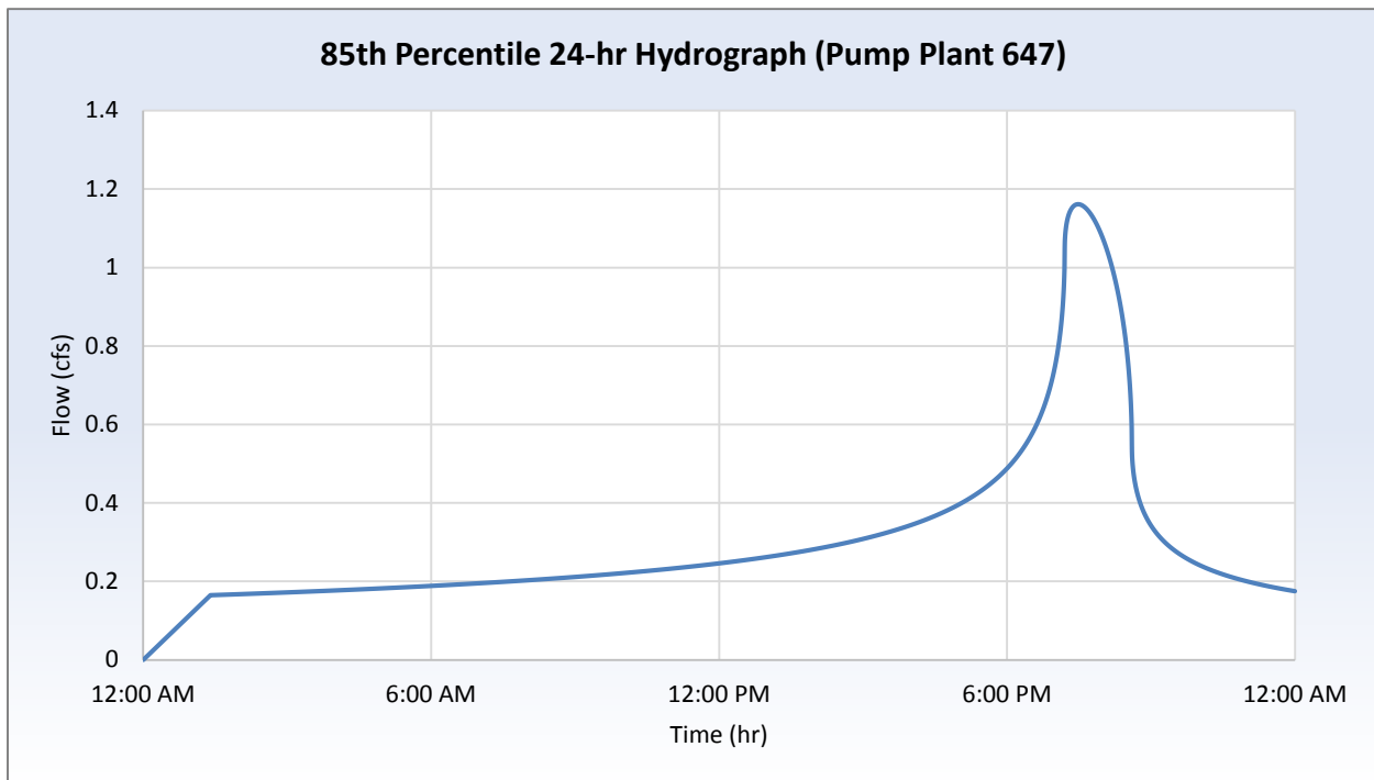
Figure 16. 85th Percentile 24-Hour Hydrograph for the 10- acre drainage area with 0.94 inch Rainfall Depth.
