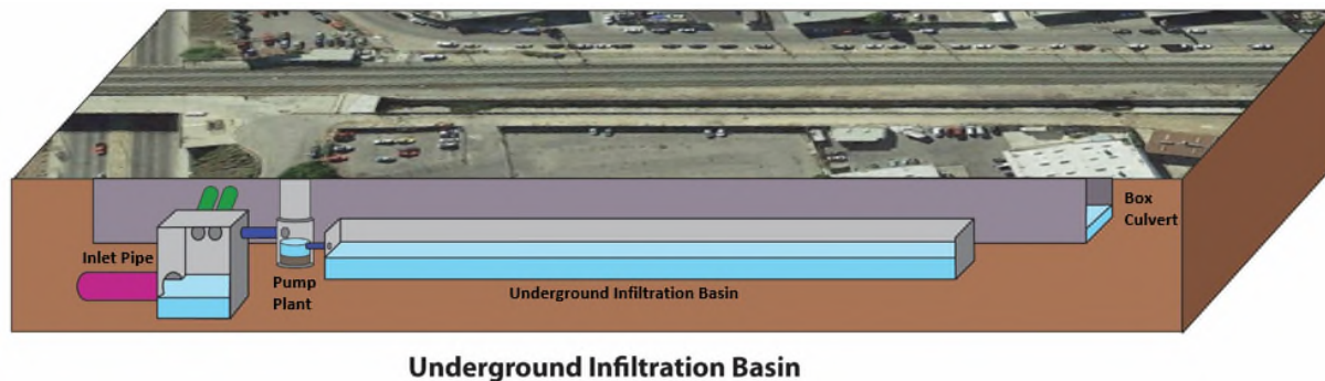
Figure 25. BMP configuration for Alternative 1, scenario 2.
