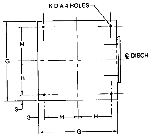
SOLE PLATE ANCHORING DIMENSIONS
