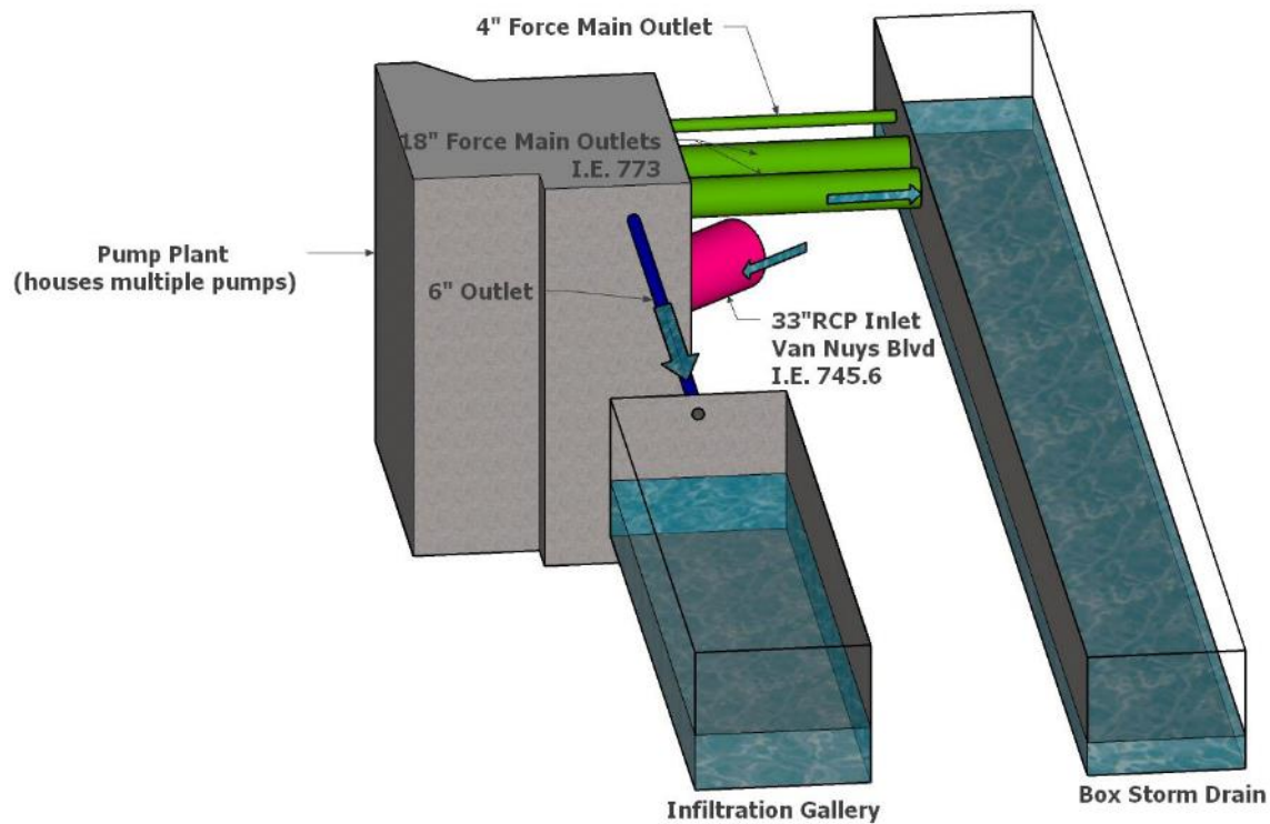
Figure 14. Direct Pumping System for Alternative 1-Scenario 2.
