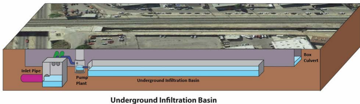
Figure 24. BMP configuration for Alternative 1, scenario 1.
