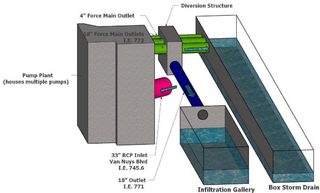
Figure 13. Weir-based Gravity Diversion System for Alternative 1-Scenario 1.
