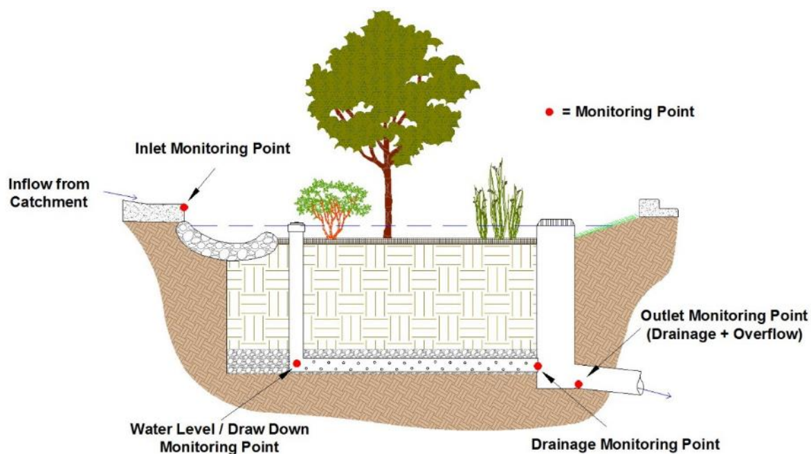
Figure 32. Typical monitoring points.
