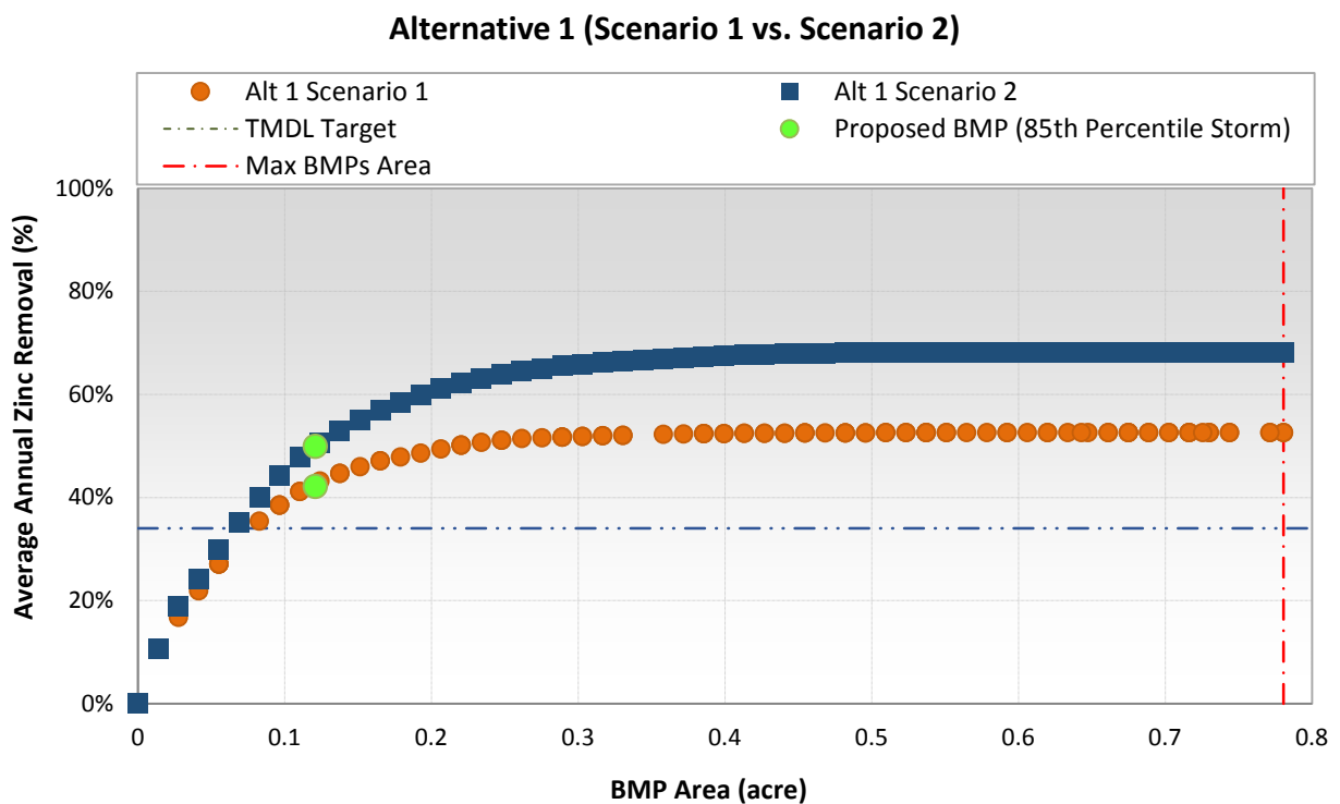
Figure 18. Comparison of water quality benefit for scenario 1 and scenario 2 (Post-Pump Treatment).
