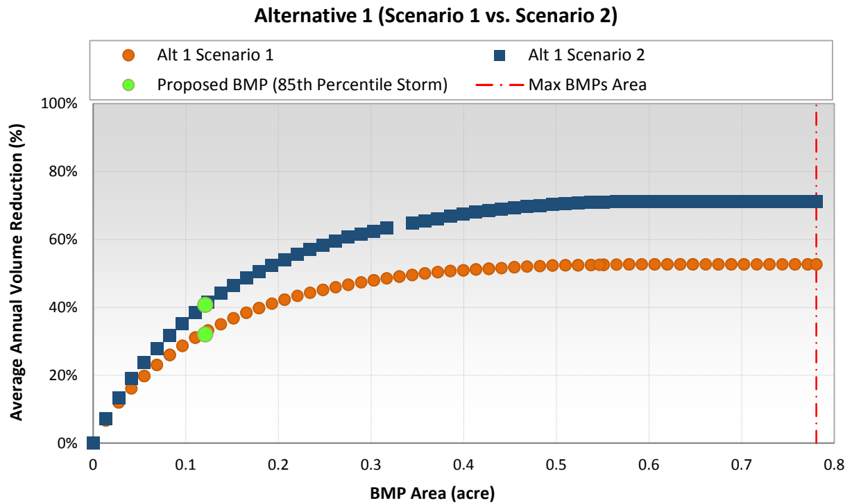
Figure 17. Comparison of 11 cfs diversion versus 1.2 cfs direct pumping for Alternative 1 (Post-Pump Treatment).
